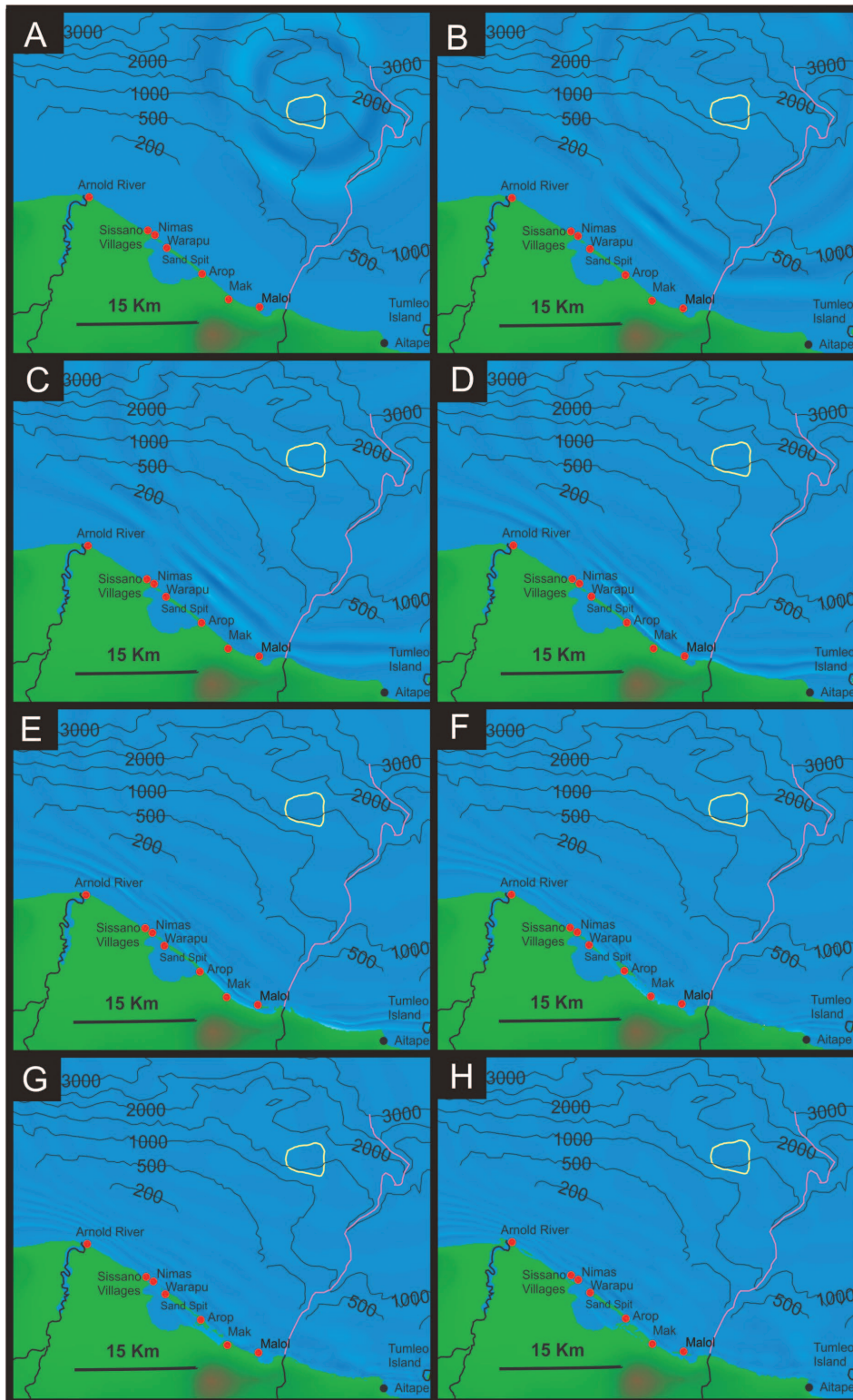
Fig. 5. Eight snapshots of tsunami propagation and inundation using FUNWAVE, a uniform 100×100 m grid spacing, and the latest slump source. Light blue are elevation waves and dark blue are depression waves. (Time after main shock; time after slump initiation). (a) [15.6 min; 3.1 min]. (b) [18.6 min; 6.1 min]. (c) [20.1 min; 7.6 min]. (d) [21.6 min; 9.1 min]. (e) [23.2 min; 10.7 min]. (f) [24.7 min; 12.2 min]. (g) [26.2 min; 13.7 min]. (h) [27.7 min; 15.2 min]. The slump location is in yellow, and Yalingi Canyon is marked in purple. See text for further discussion.
